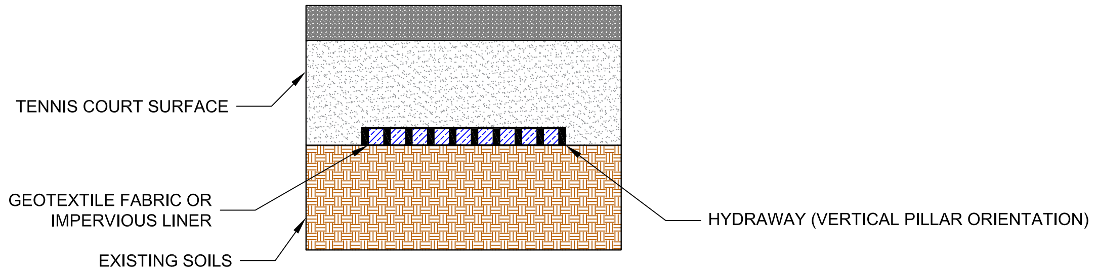
TYPICAL SUBSURFACE DRAIN DETAIL
