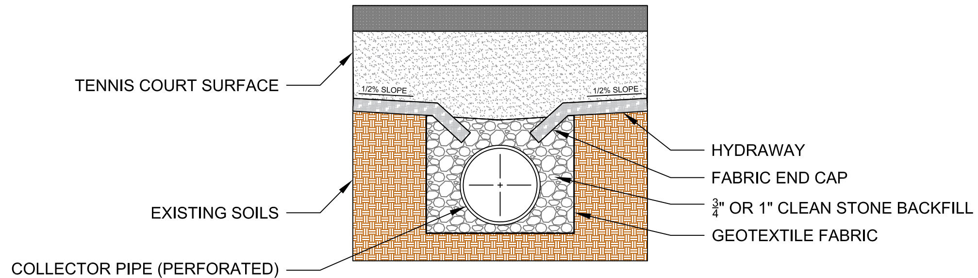
TYPICAL DRAIN TERMINATION DETAIL
