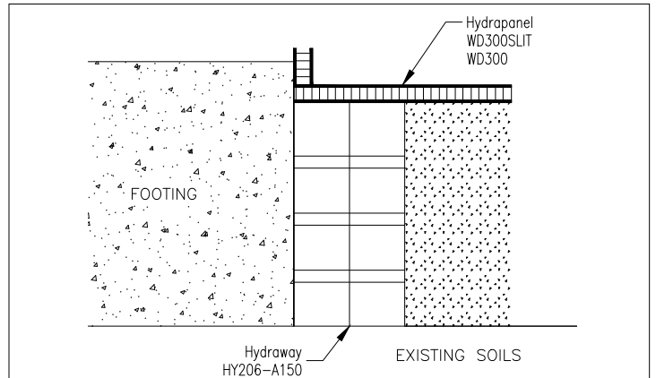
Figure 5. HydraPanel extending width of footing, plus overage.
