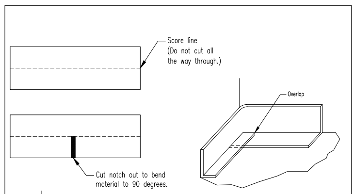
Figure 7. Installing HydraPanel at a corner.
