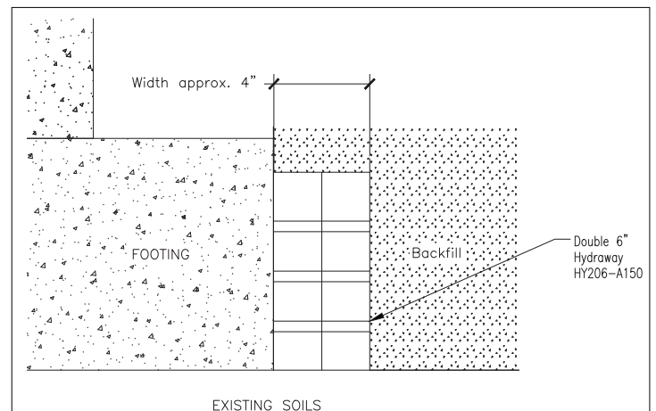
Figure 1. Double roll of 6-inch Hydraway.
